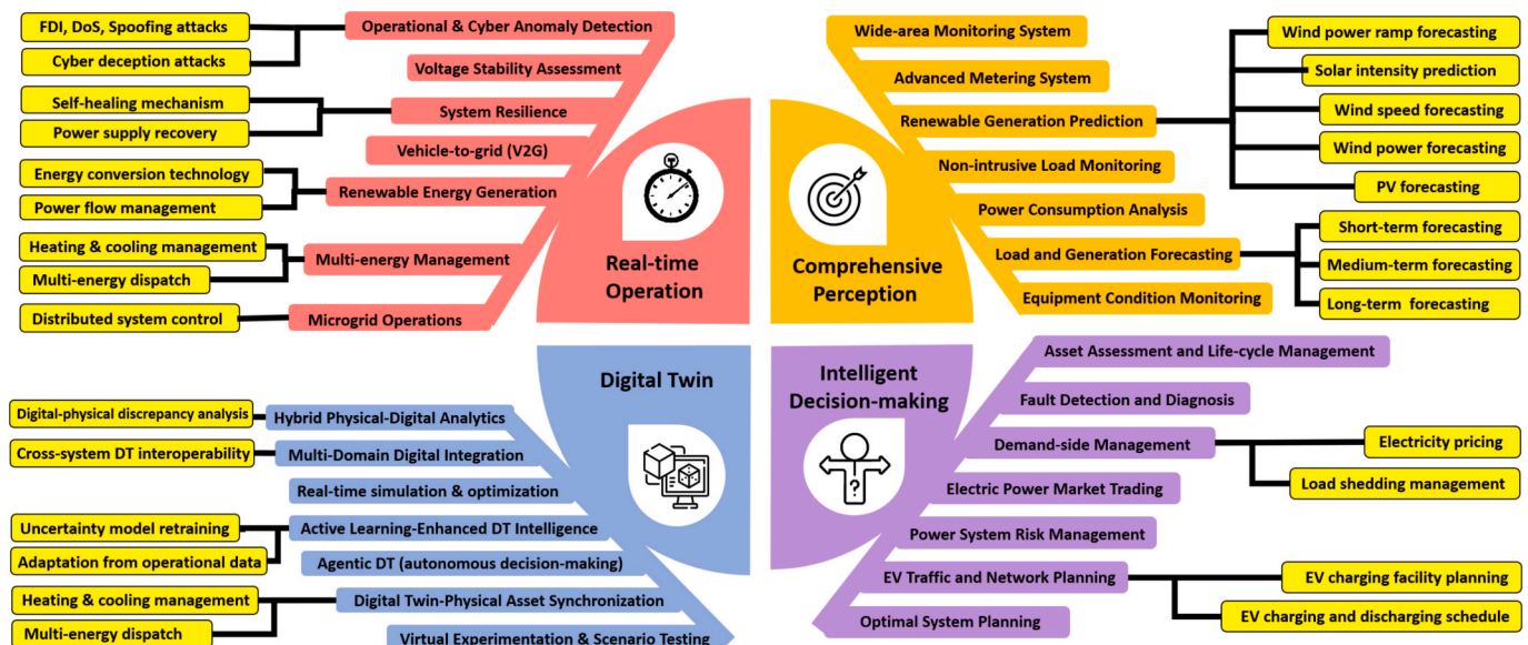
Fig. 10. Applications of AI/ML techniques in various domains of smart grids and power systems.
