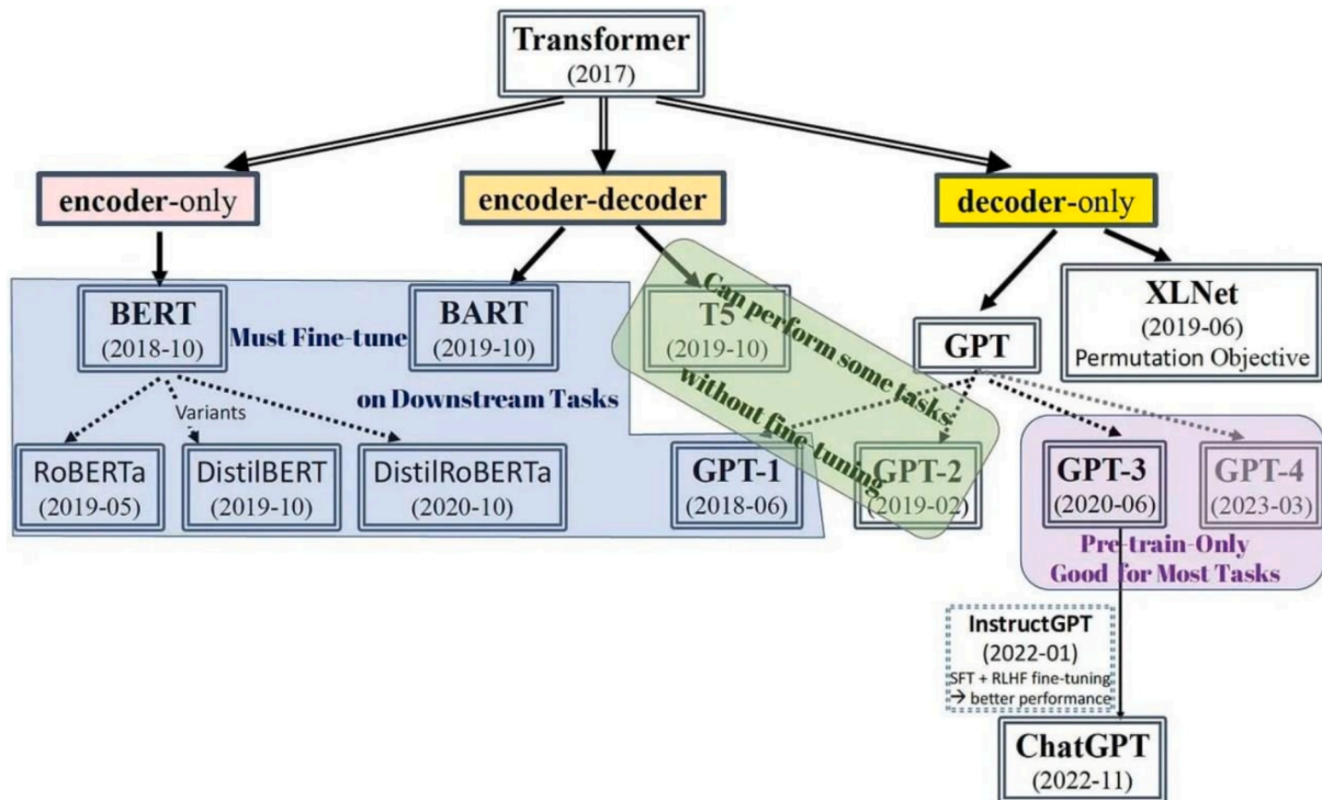
Fig. 8. Evolution of Transformer-Based Generative Architectures [55].
